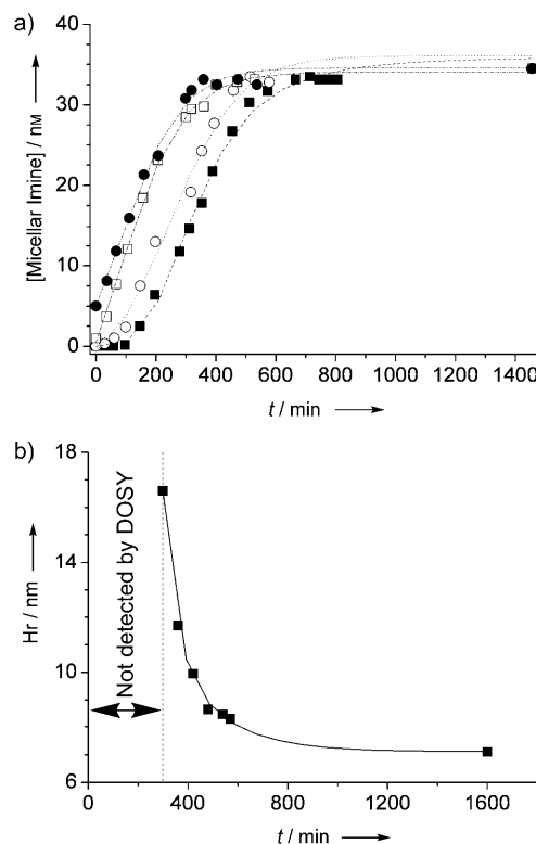
Figure 2. Autopoietic behavior of dynablock 7A . a) Concentration of micellar imine 7A versus time starting from 7 and A in D_2O (50 mM each), and as a function of the quantity of initially added micellar imine 7A : \blacksquare 0, \circ 5.1 \times 10^{-4} , \square 51 \times 10^{-4} , \bullet 102 \times 10^{-4} mmol. The micelle concentrations were determined by the integration of the micellar imine ^1H NMR spectroscopy signal (8.12 ppm), which differs from the free imine signal (8.23 ppm). Maximum standard deviation of the data presented 5%, determined by setting up the reaction three times under the same conditions. Dotted lines connecting the experimental results drawn to guide the eye. b) Hydrodynamic radii H_r of the micellar structure formed from 7A as a function of the course of the condensation reaction from 7 and A .
